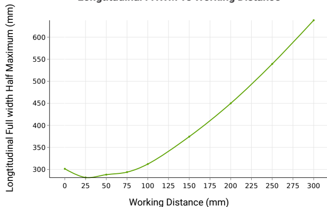
Longitudinal FWHM vs Working Distance
