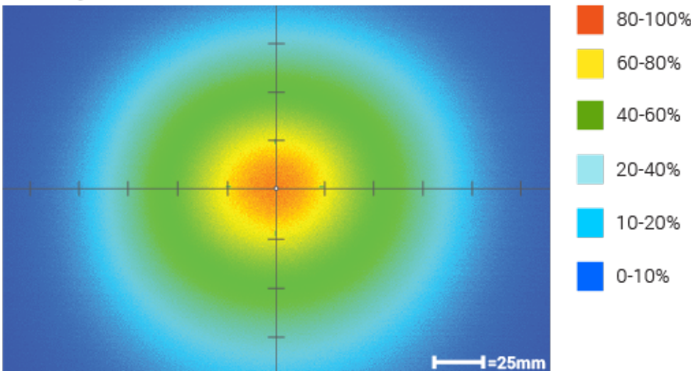
Optical measurement taken using SL-S050075M-WHI @ 300 mm
